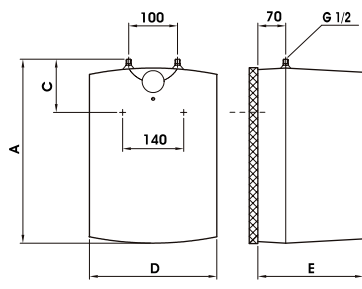
UNDERSINK DESIGN
