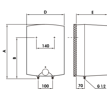
OVERSINK DESIGN
